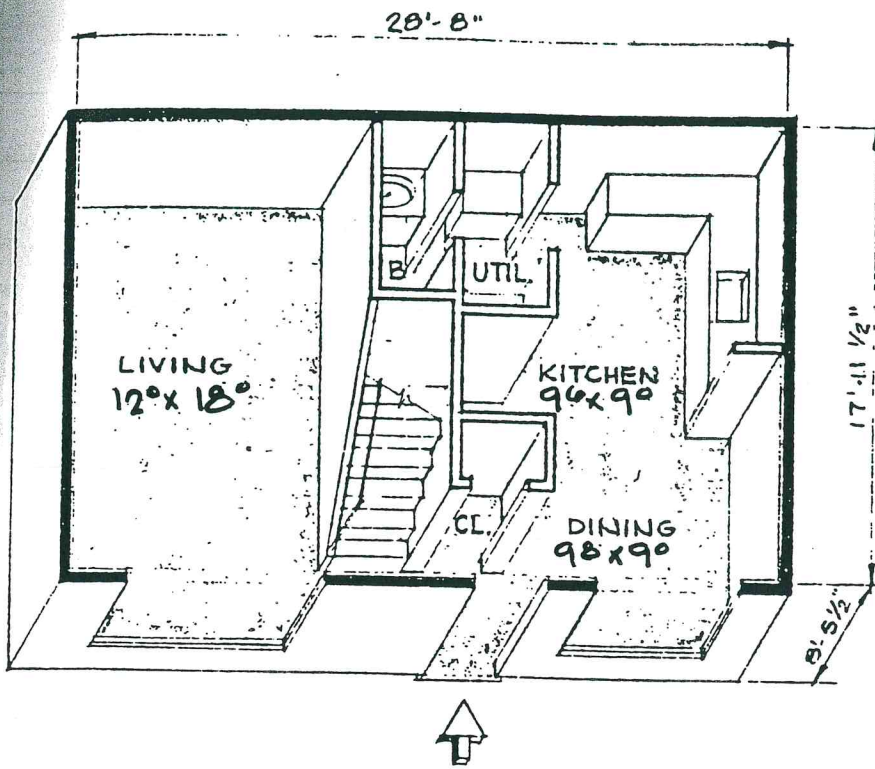
UNIT 'B' FIRST FLOOR
