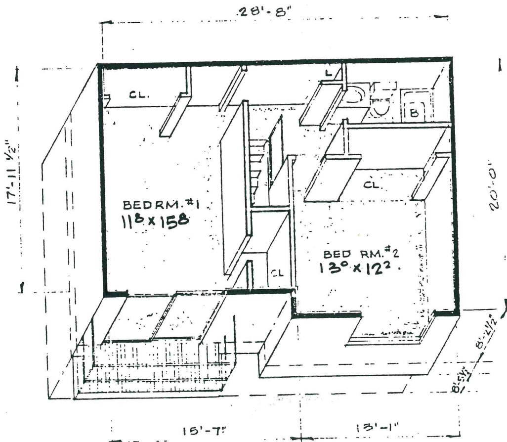
UNIT 'B' SECOND FLOOR
