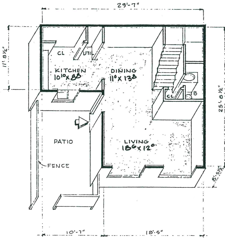
GROUND FLOOR UNIT 'C'
